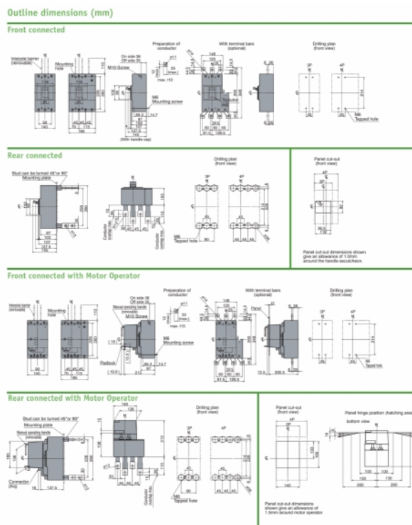
Dimension Diagram
