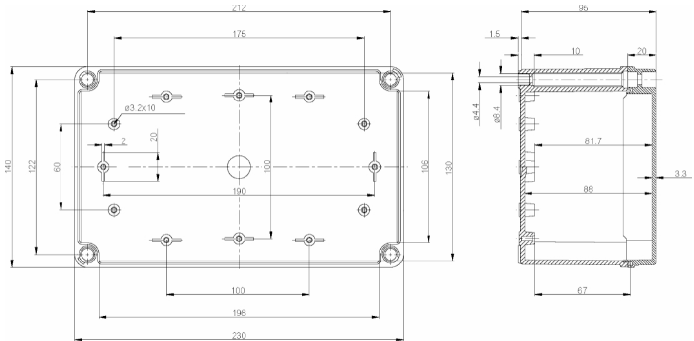
Dimension Diagram
