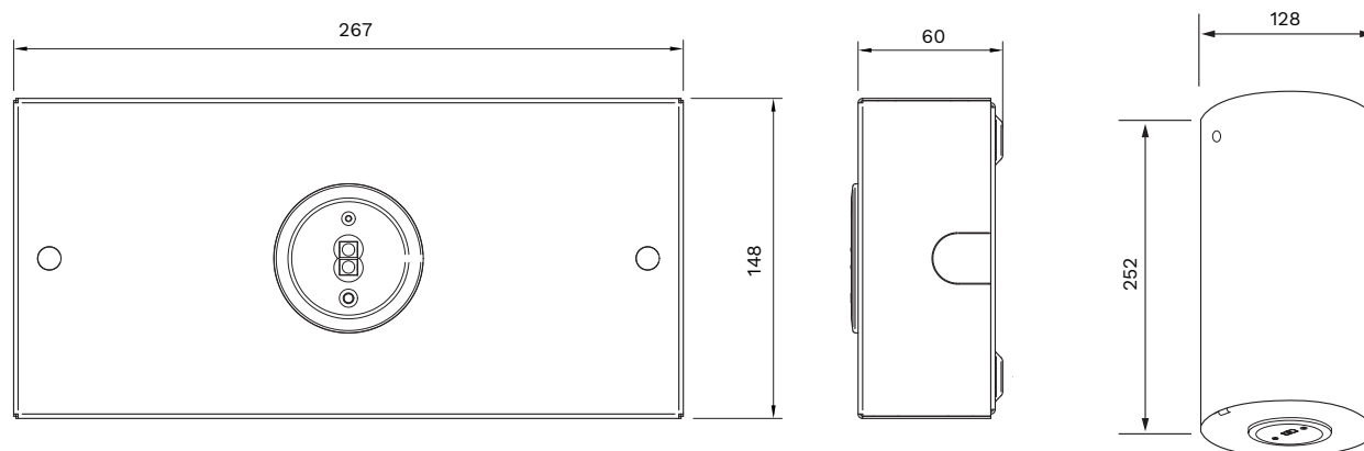
Dimensions (mm)
