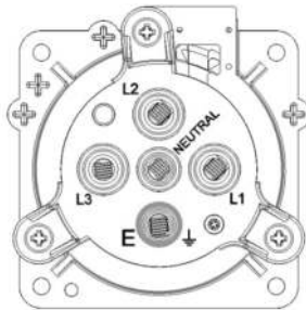
4 & 5 Round pin
