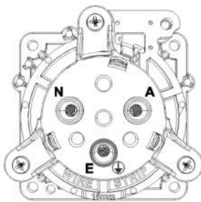
3 Round pin
