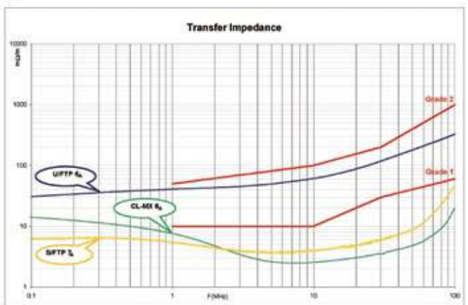
CL-MX transfer impedance graph
